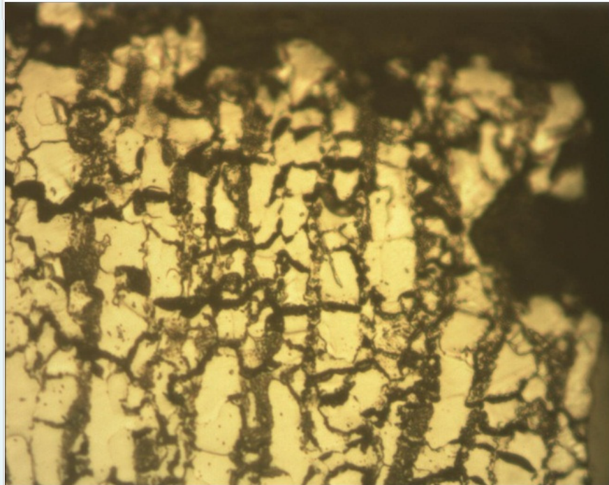
Microstructure shows presence of fissures from ID due to HTHA
