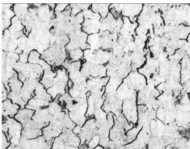
Figure 2b. SEM micrograph showing the final stage of formation fissures and micro-cracks.
