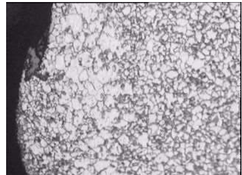
Figure 3 Shows effect of grain coarsening at OD edge on a 660MW Boiler's Water wall tube. The material of construction is SA213 Grade T22. Microstructure shows ferrite and grain boundary pearlite. (200X)
